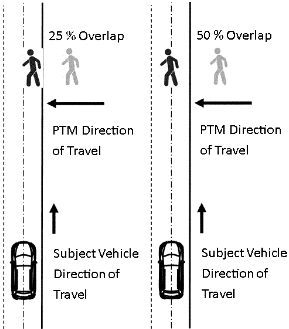
Figure 3 to § 571.127—Setup for Pedestrian, Crossing Path, Right
